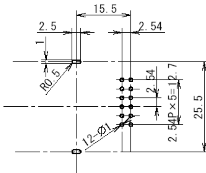
Reference hole position (Top view)
